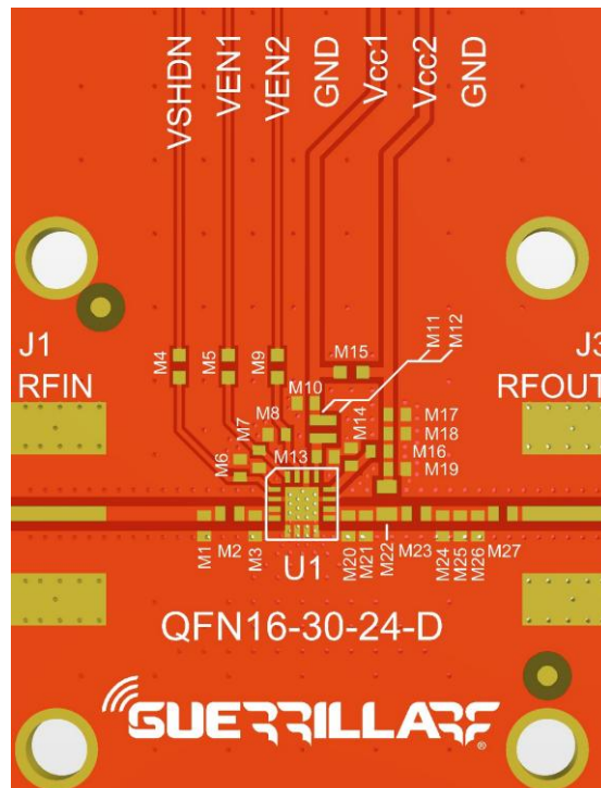
GRF5507 Evaluation Board Assembly Diagram
