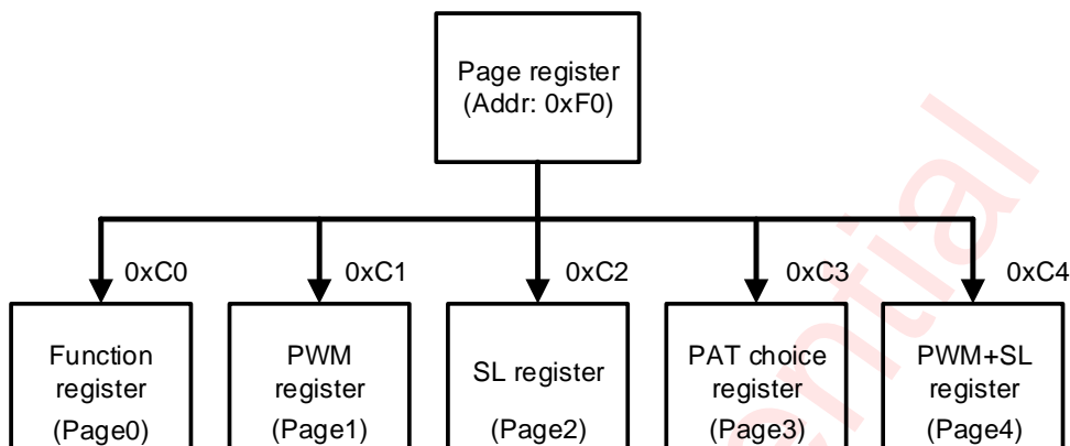
Figure 23 Register Control
