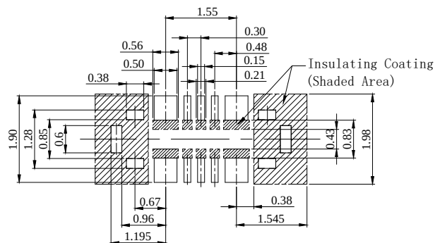
RECOMMENDED PCB LAYOUT DIMENSIONAL TOLERANCE: ±0.02
