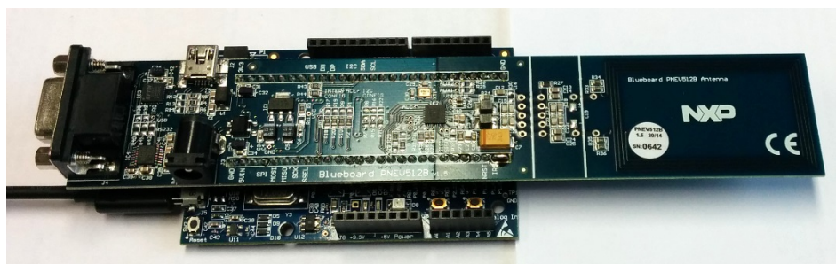
Fig 14. CLEV663B connected to LPCXpresso LPC11U68 development board
