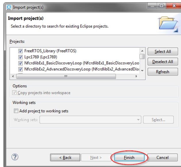
Fig 24. Importing a project into the LPCXpresso IDE
