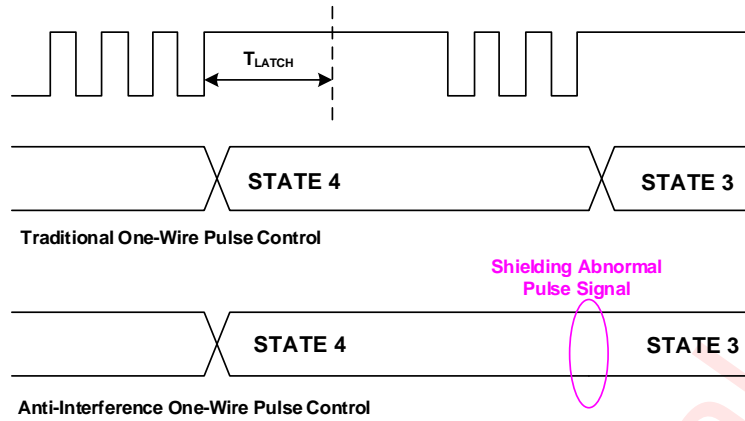
Figure 15 Anti-Interference One-Wire Pulse Control Functional Diagram
