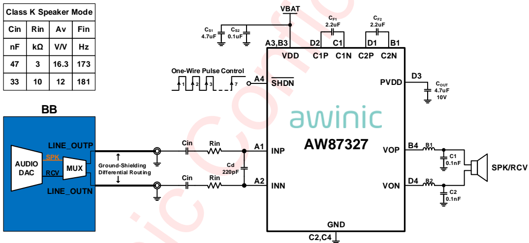
Figure 5 AW87327 Differential Input Speaker Mode Application Diagram
