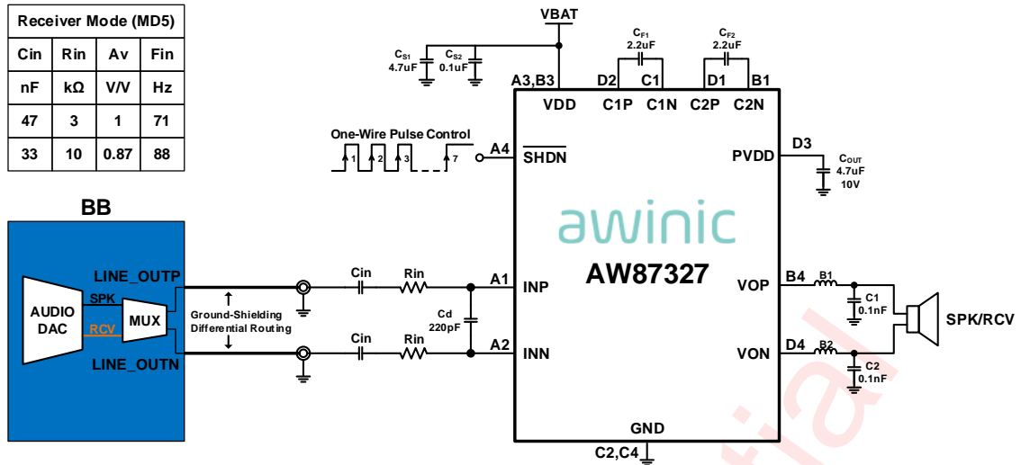
Figure 7 AW87327 Differential Input Receiver Mode Application Diagram
