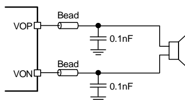
Figure 19 Ferrite Beads and Filter Capacitors
