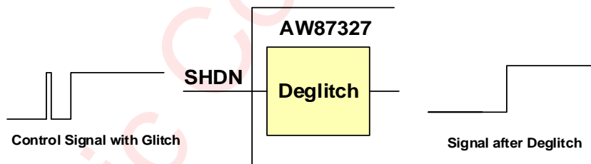
Figure 14 AWINIC Deglitch Working Principle
