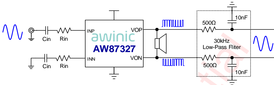
Figure 8 AW87327 Test Setup
