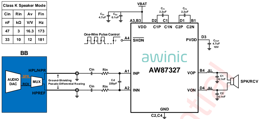
Figure 4 AW87327 Single-ended Input Speaker Mode Application Diagram (Note 1)
