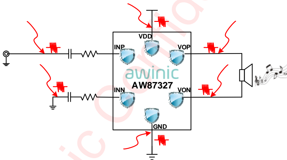
Figure 18 AW87327 Rejection of RF Noise
