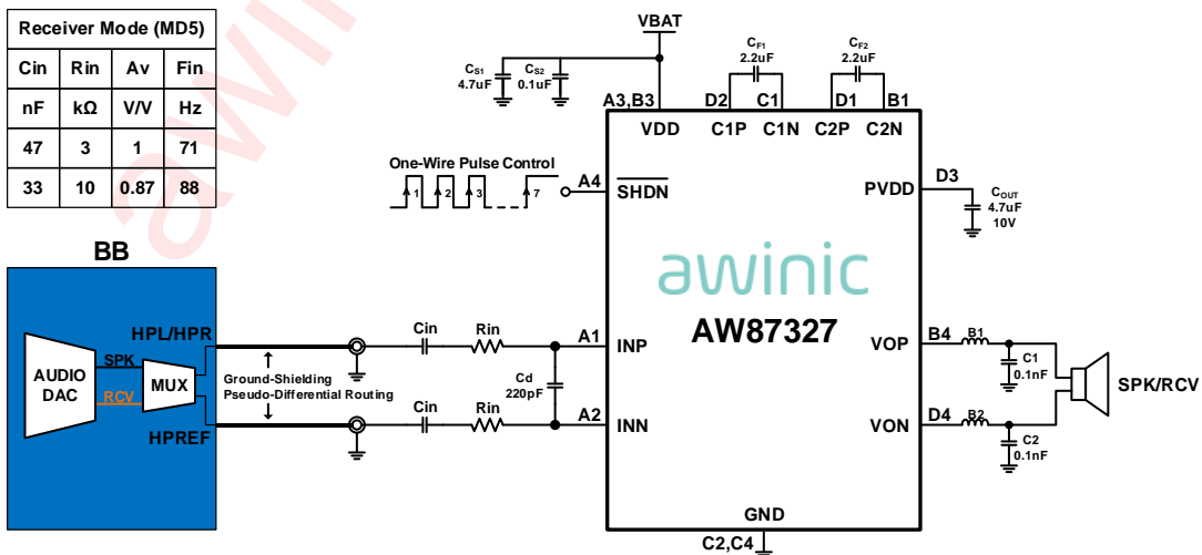
Figure 6 AW87327 Single-ended Input Receiver Mode Application Diagram
