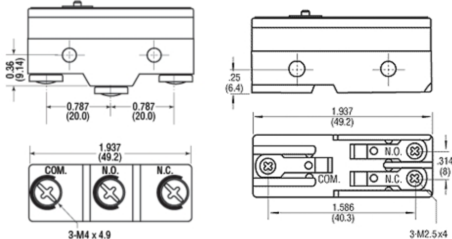
Screw Terminal
