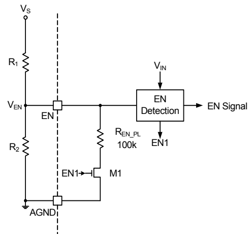
Figure 2. Enable Internal Circuit of AOZ2253TQI-20
