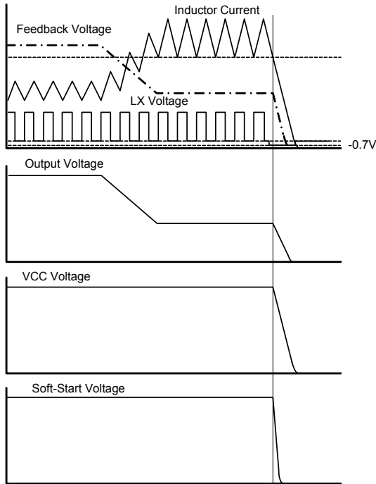
Figure 5. OCP Timing Chart of AOZ2253TQI-20
