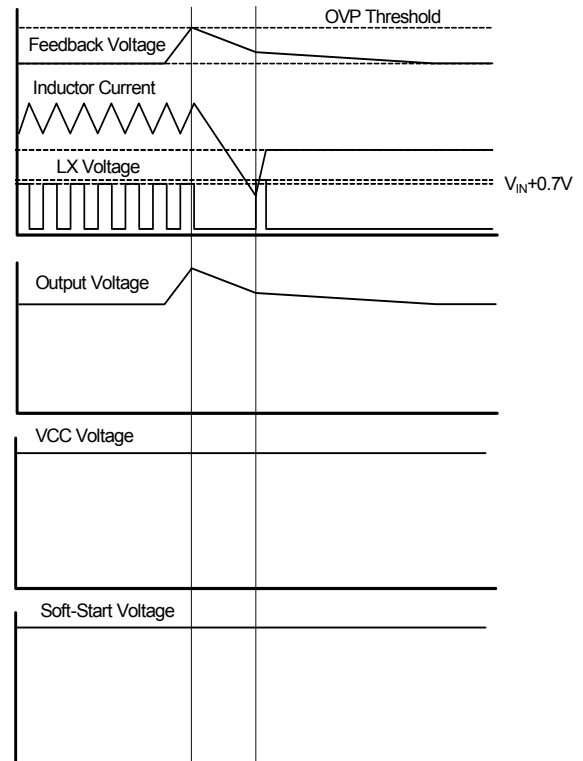
Figure 6. OVP Timing Chart of AOZ2253TQI-20
