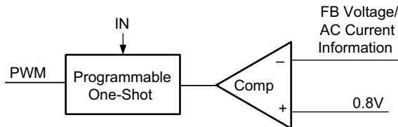
Figure 4. Simplified Control Schematic of AOZ2253TQI-20
