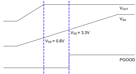
Figure 1. Soft Start Sequence of AOZ2253TQI-20
