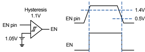
Figure 3. Enable Threshold Schematic and Timing Sequence of AOZ2253TQI-20
