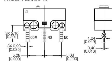
TYPE 30 - PCB SNAP-IN
