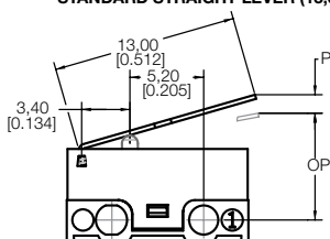
TYPE C STANDARD STRAIGHT LEVER (13,0 mm)
