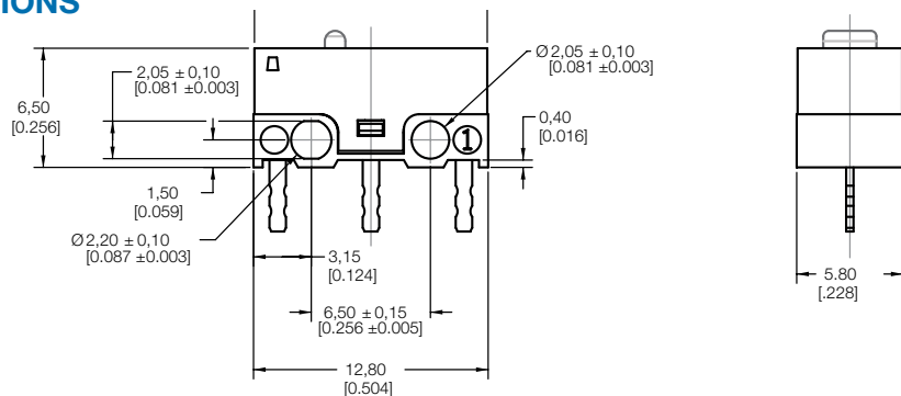
TYPE 20 - PCB STRAIGHT
