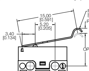
TYPE H SIMULATED ROLLER LEVER (15,0 mm; R1,3)
