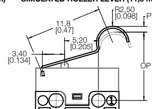
TYPE E SIMULATED ROLLER LEVER (11,8 mm; R2,5)
