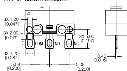
TYPE 10 - SOLDER STRAIGHT
