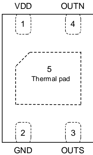
AW86510EDCBDNR Top View
