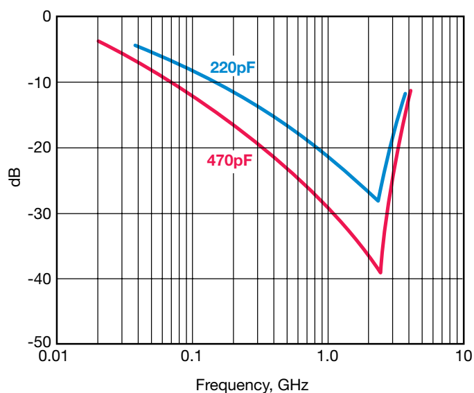
S21 vs. Frequency X7R 4 Element Feedthru
