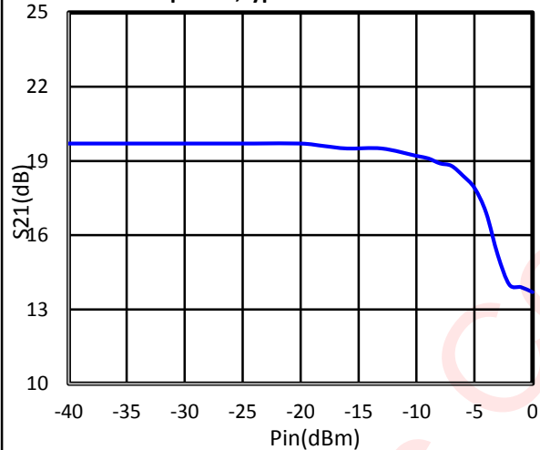
OOB P-1dB as a function of input power;typical values
