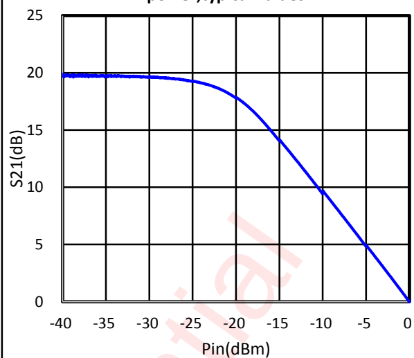
IB P-1dB as a function of input power;typical values
