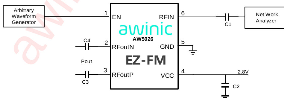
Figure 10 AW5026 Tunable Capacitor Measurement Diagram
