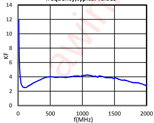
Stability Factor as a function of frequency;typical values
