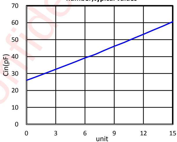
Tunable Capacitor as a function of pulse number;typical values
