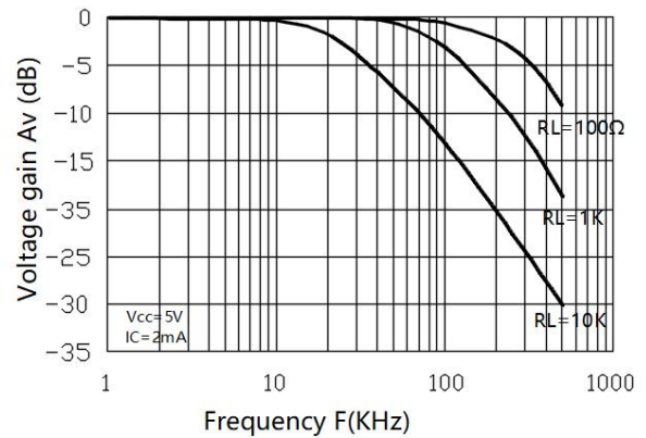
Fig.10 Frequency Response
