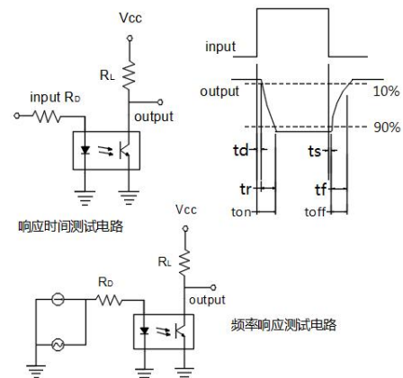
Fig.12 Switching Time Test Circuit & Waveforms
