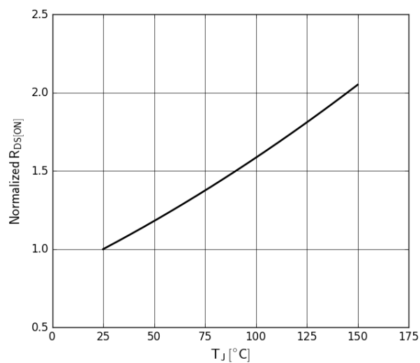
Figure 4. Normalized On-resistance
