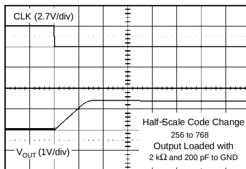
HALF-SCALE SETTLING TIME
