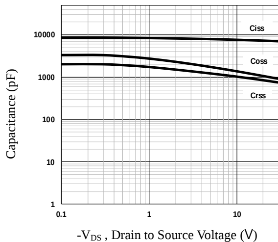
Fig.7 Capacitance Characteristics
