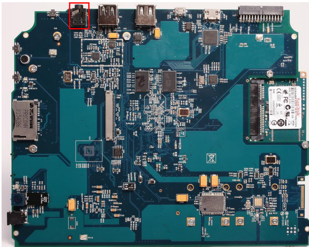
Figure 4-3. Headphone Connector
