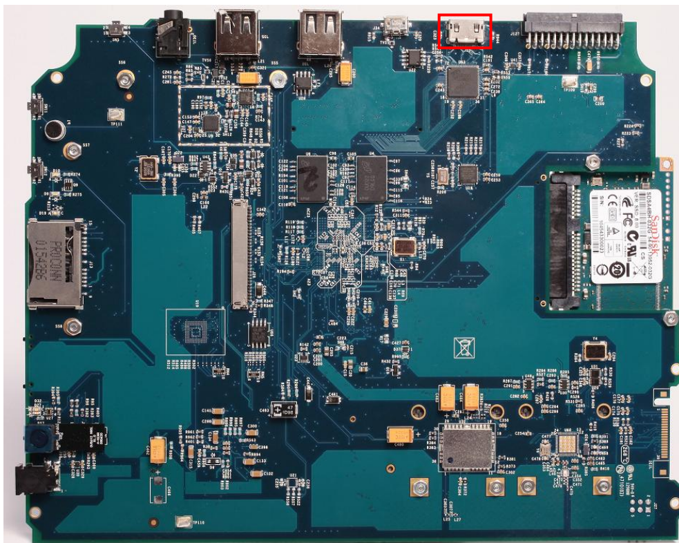
Figure 4-6. Mini-HDMI Connector
