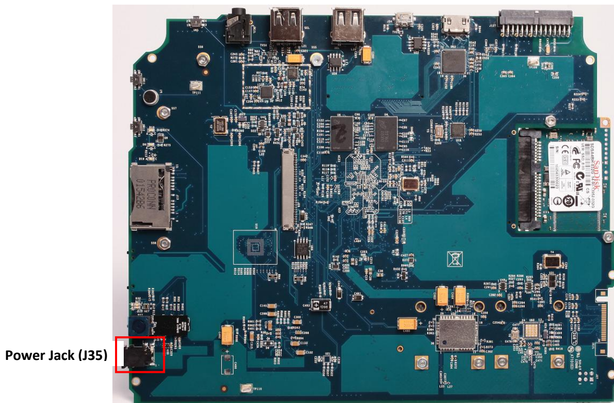
Figure 4-1. DC Power Jack
