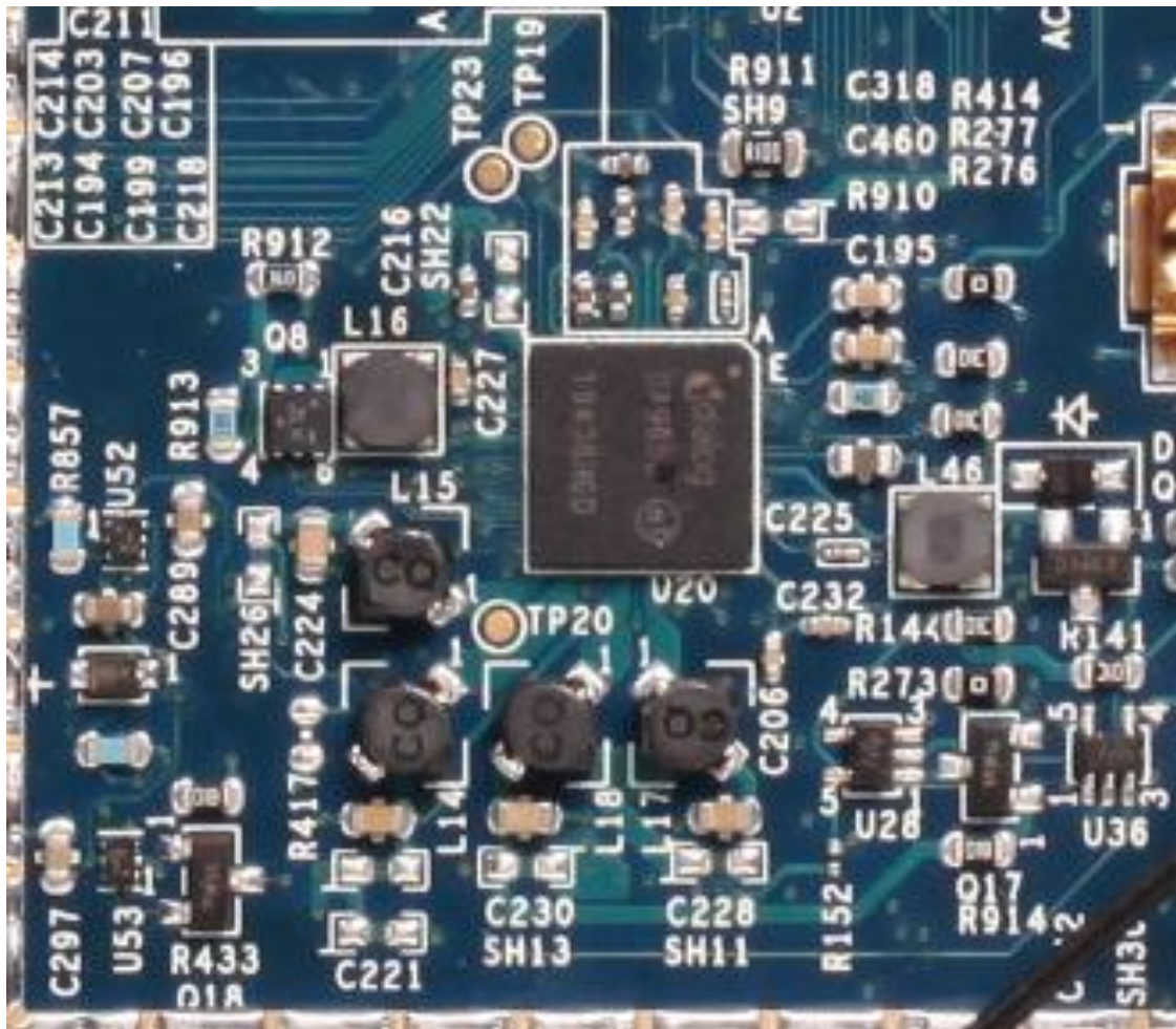
Figure 10-1. Regulator Output Capacitor Positions Top
