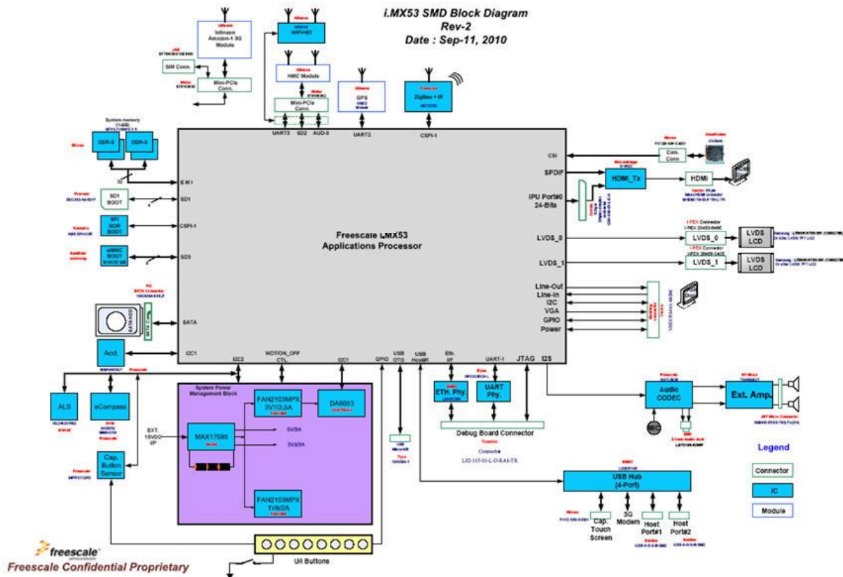
Figure 5-1. MCIMX53SMD Board Block Diagram
