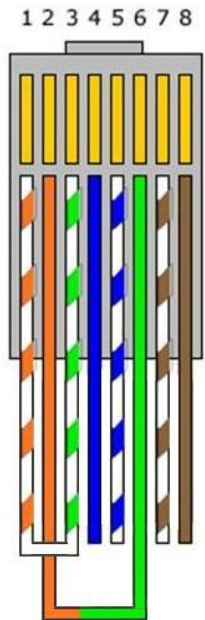
Figure 9-1. Ethernet Loopback Cable
