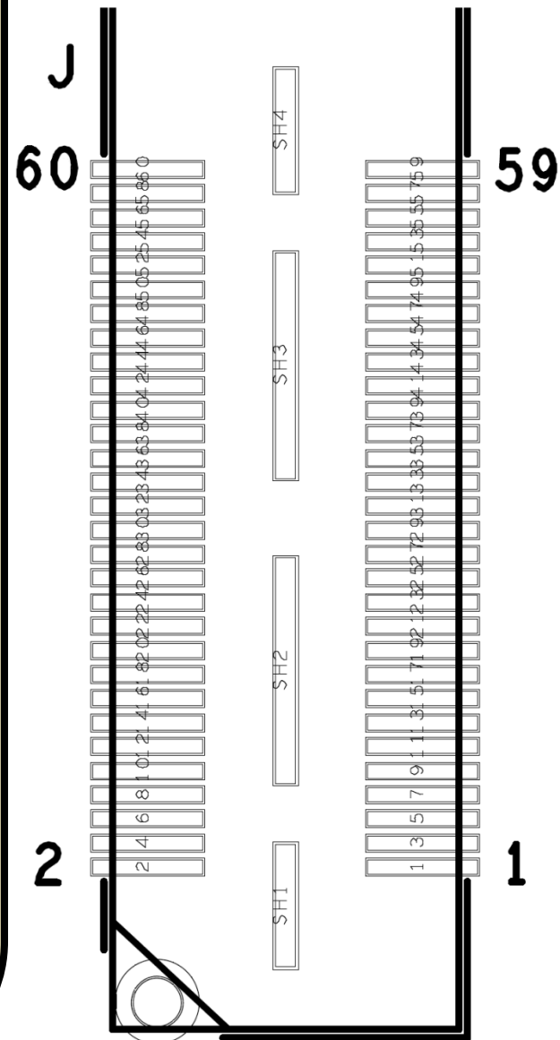
Figure 6-14. Expansion Port (J78)
