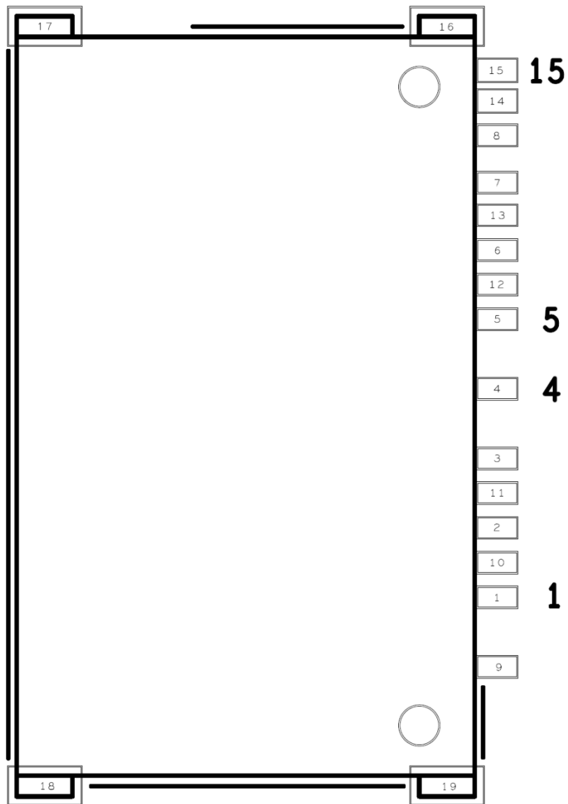
Figure 6-9. SD Card Connector (J13)
