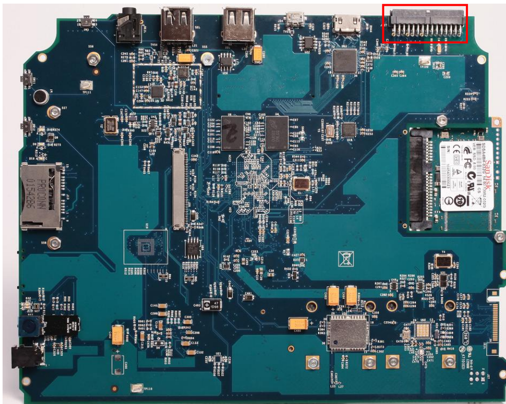
Figure 4-7. Debug Connector
