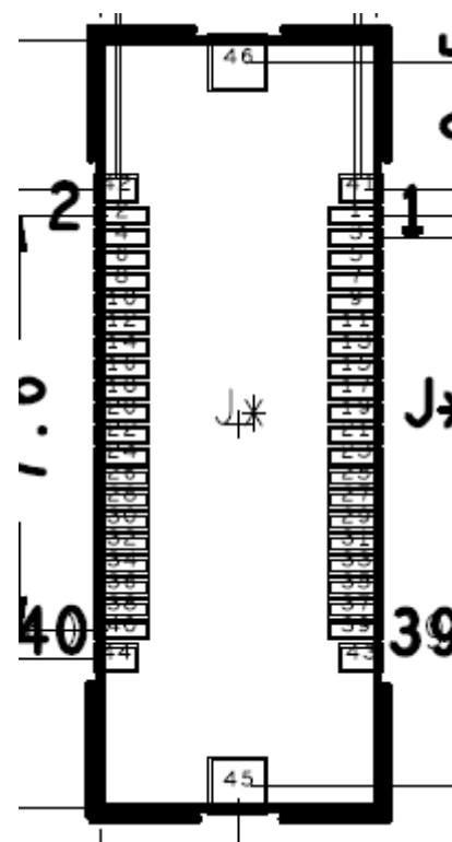
Figure 6-5. CMOS Camera Connector (J12)
