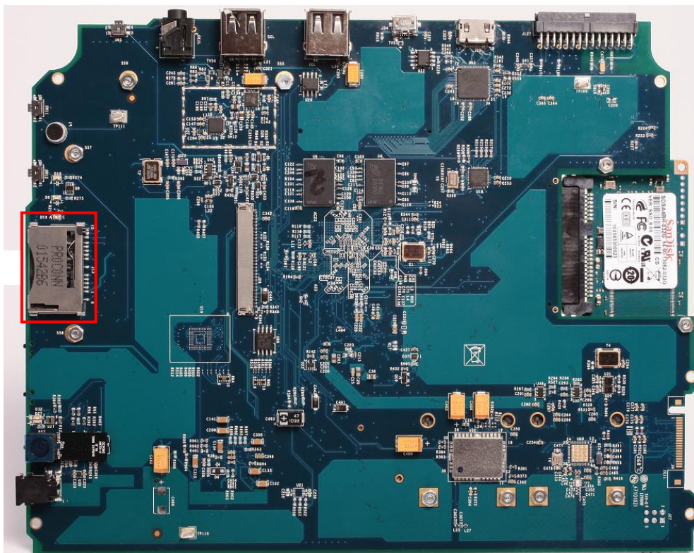
Figure 4-2. SD Connector
