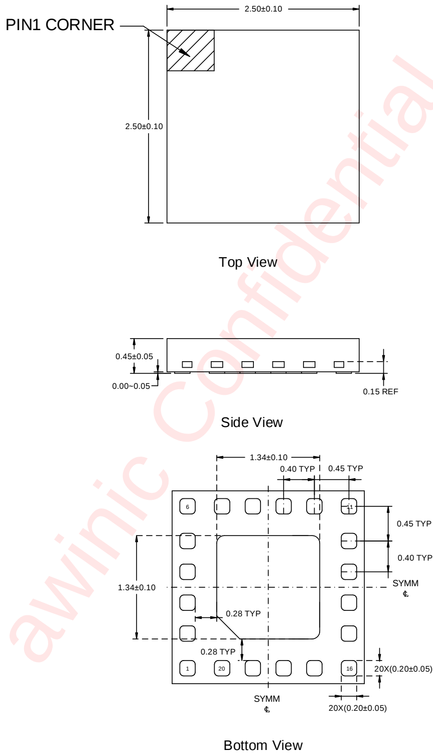
Figure 12 Package Outline
