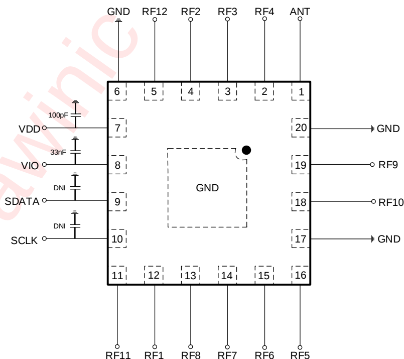
Figure 1 Typical Application Circuit of AW13512
