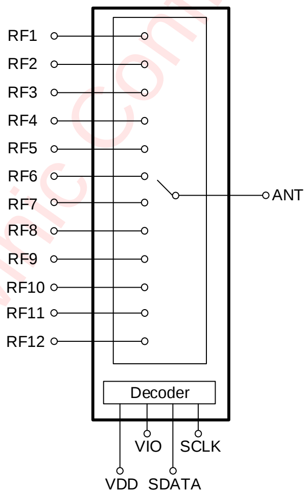
Figure 3 Functional Block Diagram
