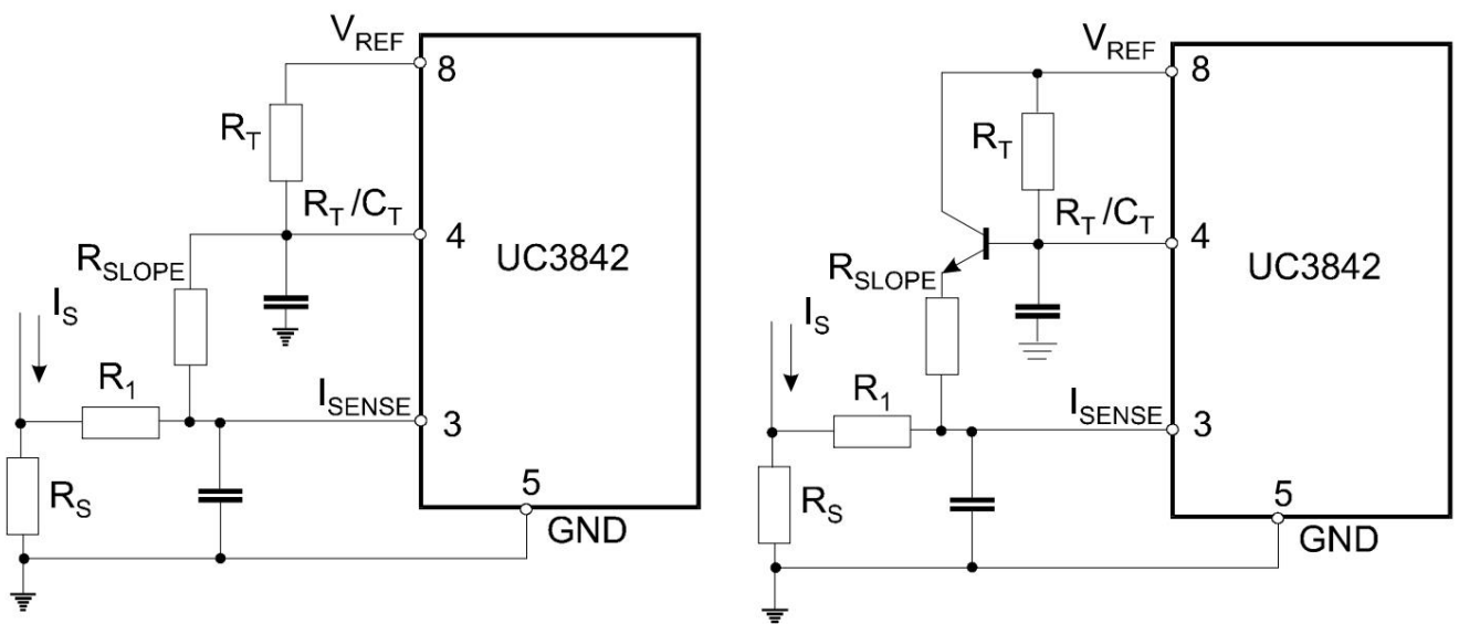
Figure 3. Current Sense Circuit
