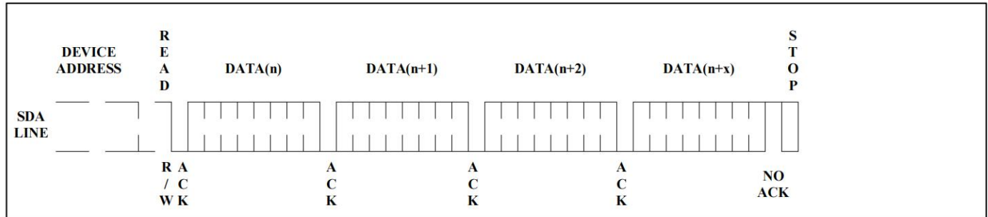
Figure 10. Sequential Read
