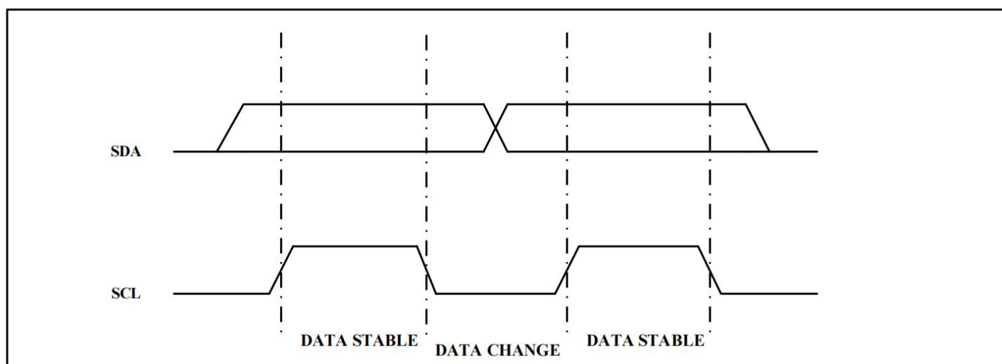
Figure 2. Data Validity
