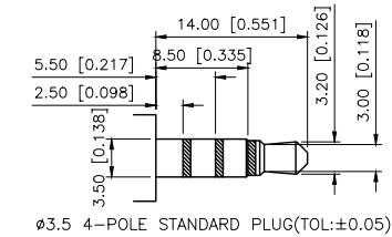
ø3.5 4-POLE STANDARD PLUG(TOL:±0.05)
