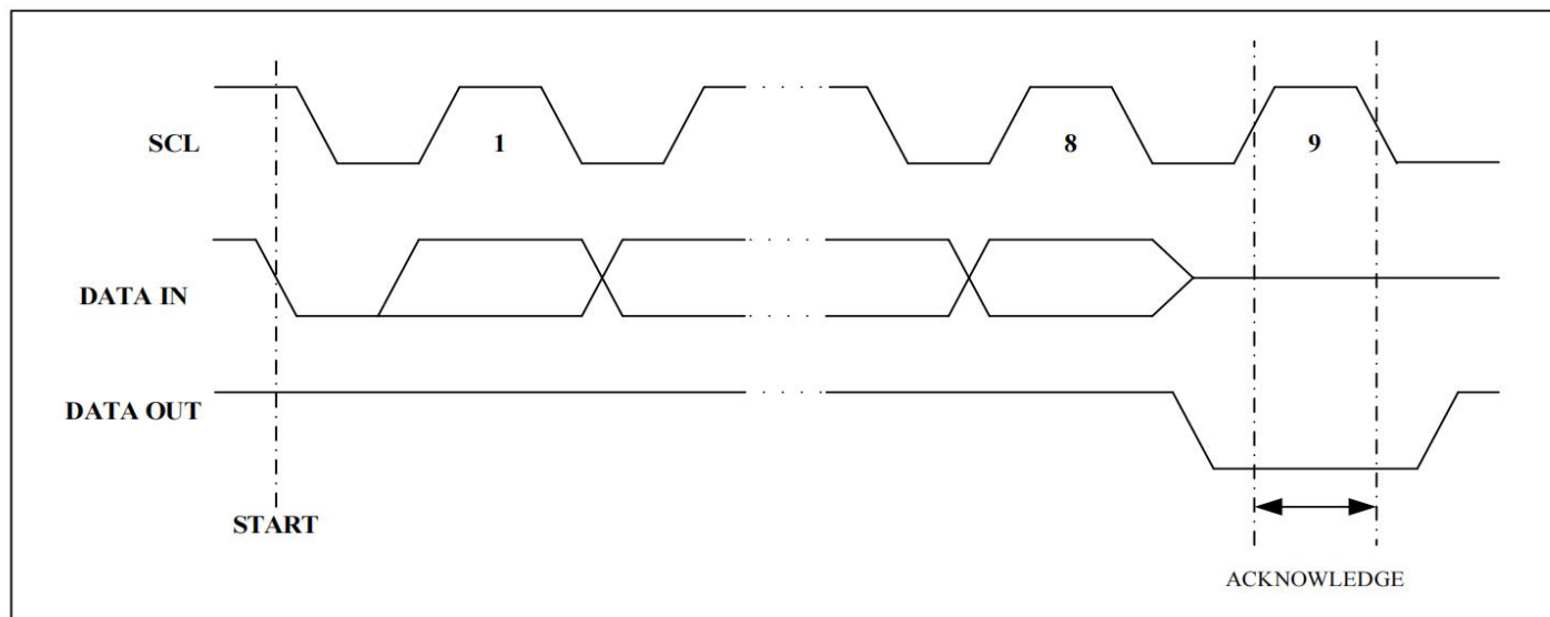
Figure 4. Output Acknowledge
