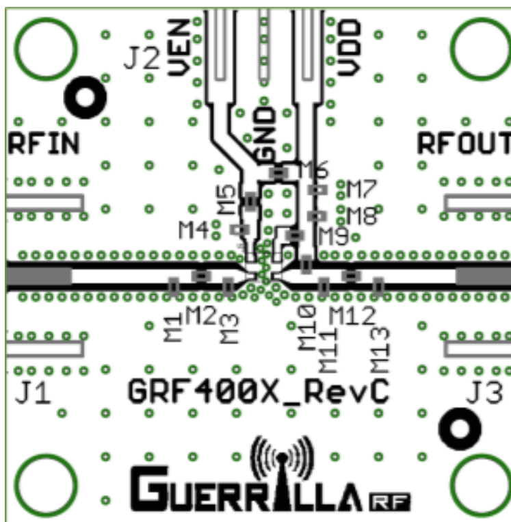
GRF2043 Evaluation Board Assembly Diagram
