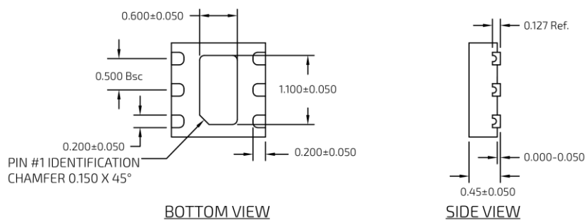
DFN-6 1.5 x 1.5 mm DFN-6 Package Dimensions
