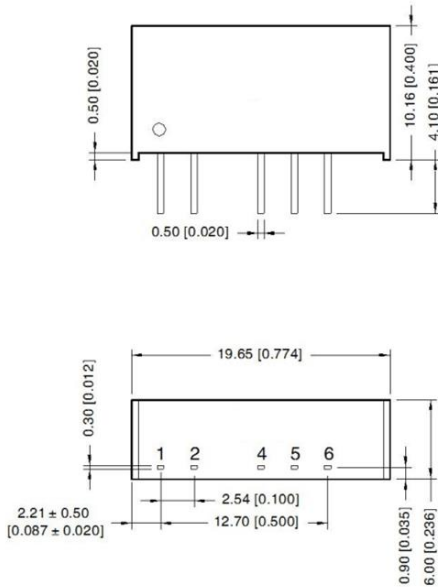
Figure 7: Overall dimensions 图7：外形尺寸
