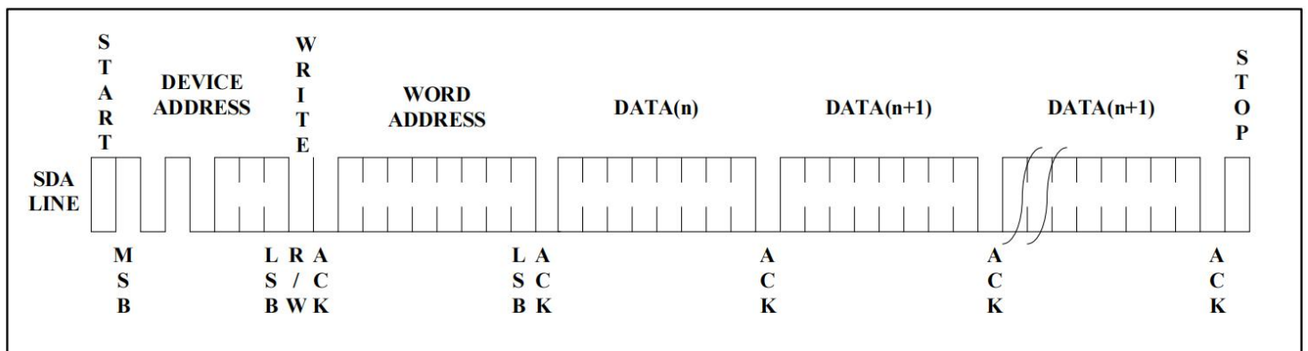
Figure 7. Page Write
