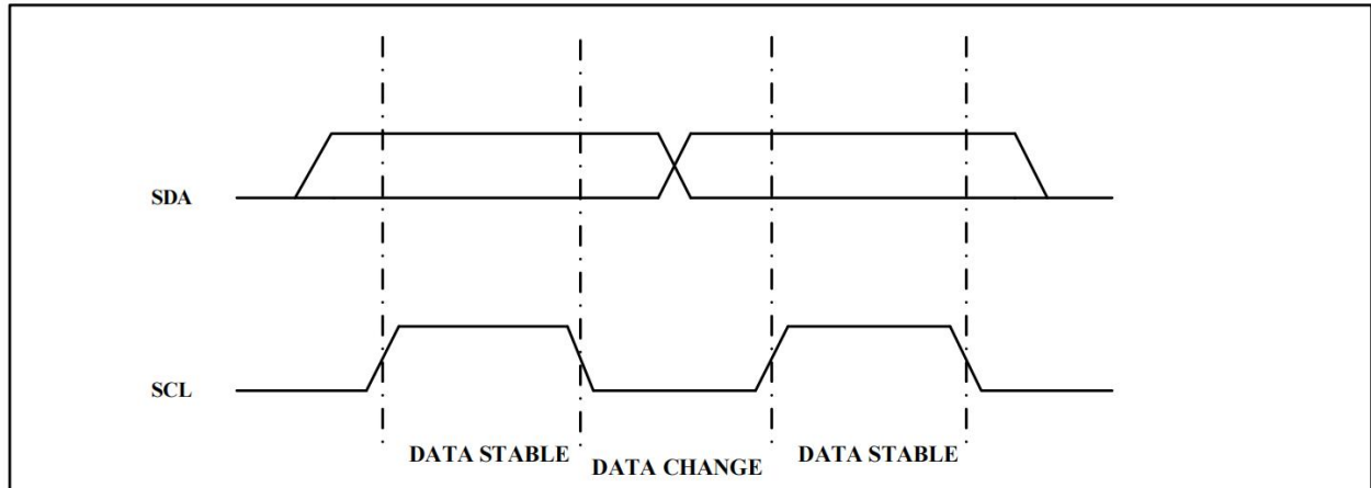
Figure 2. Data Validity
