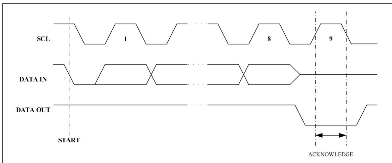
Figure 4. Output Acknowledge
