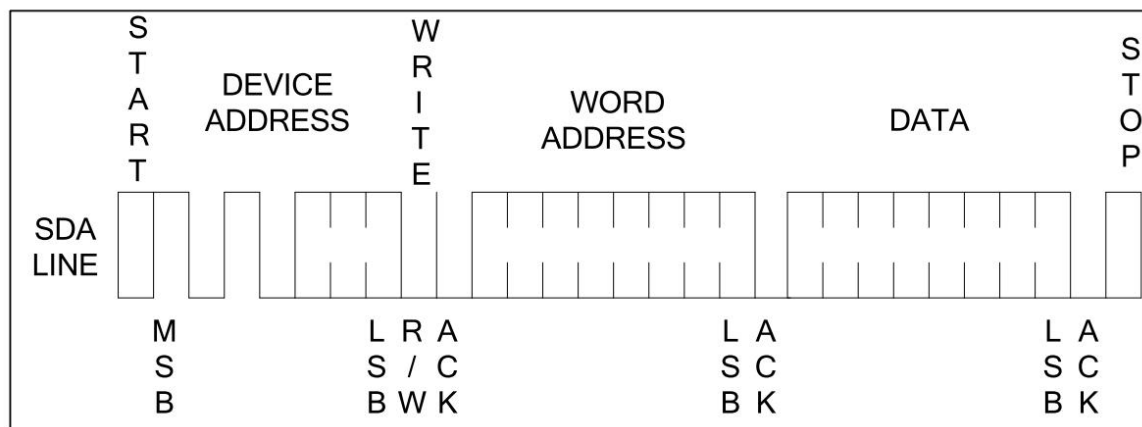
Figure 7. Page Write
