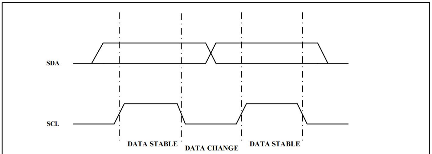
Figure 2. Data Validity
