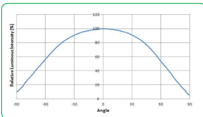
Radiation Diagram for all "XO" product
