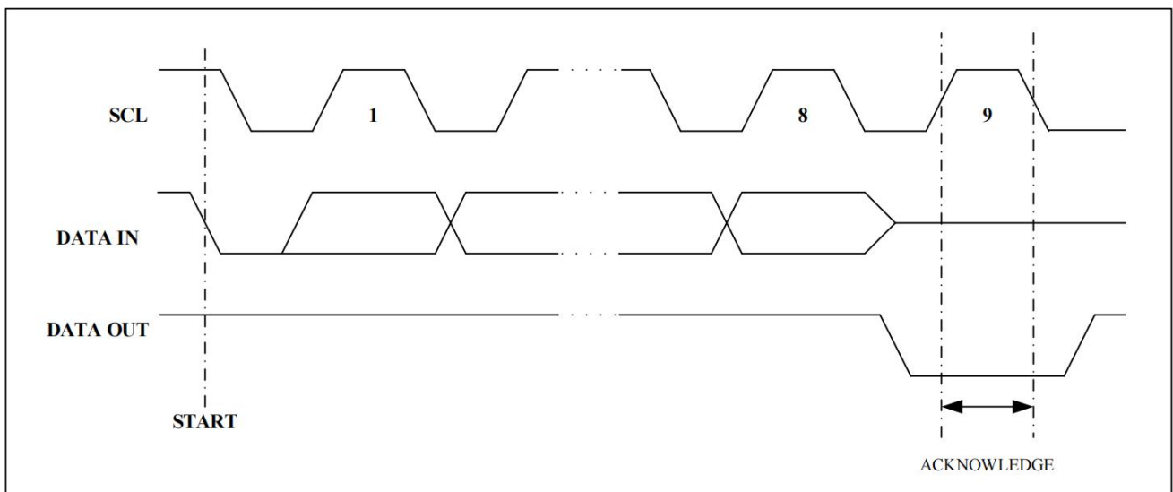
Figure 4. Output Acknowledge
