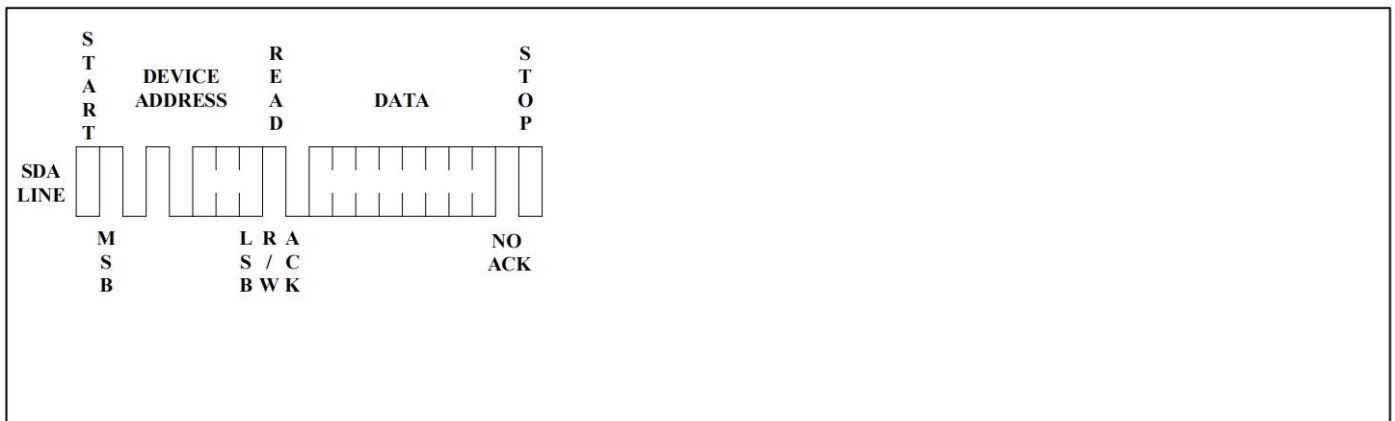
Figure 9. Random Read
