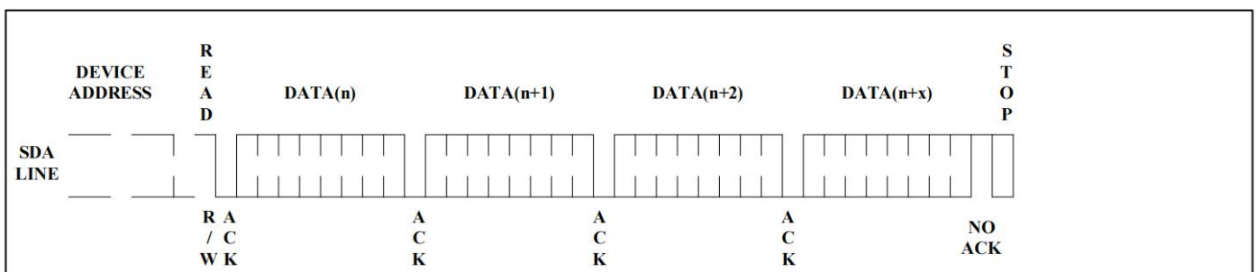
Figure 10. Sequential Read
