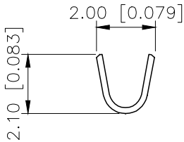
SECTION:B-B SCALE:1:1
