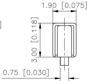
SECTION:C-C SCALE:1:1
