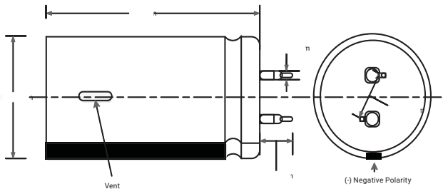
Solder Pin Type 2 pin 100F, 200F Part
