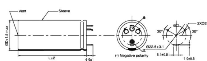
Solder Pin Type 4 pin 300F, 400F Part
