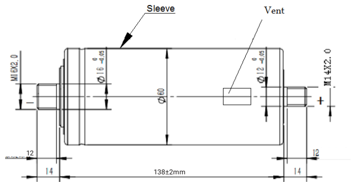
Cylindrical Screw Type 3000F Part
