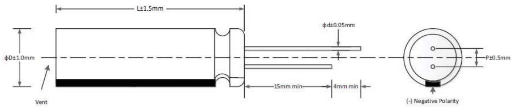
Radial Lead Type 1F – 100F
