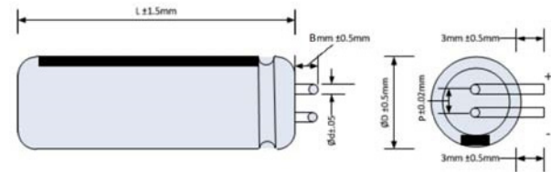
Radial Bent Lead Type
