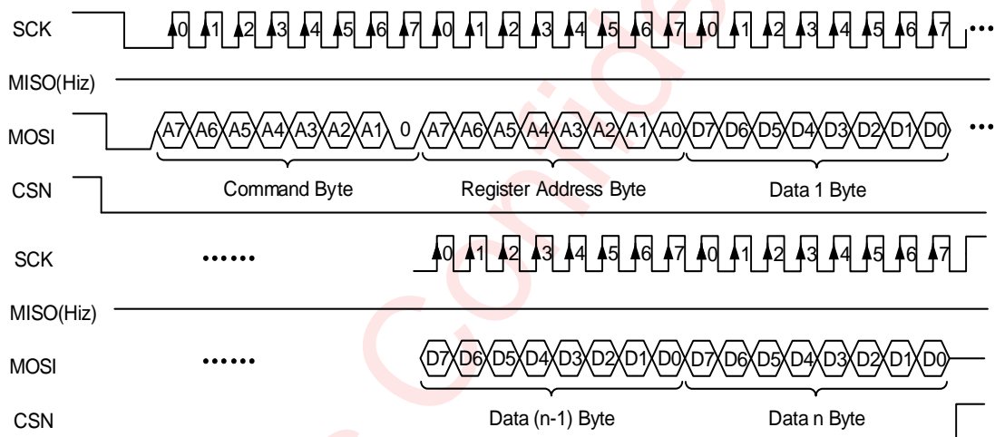
Figure 12 SPI Writing to AW20198SG (Automatic Address Increment)
