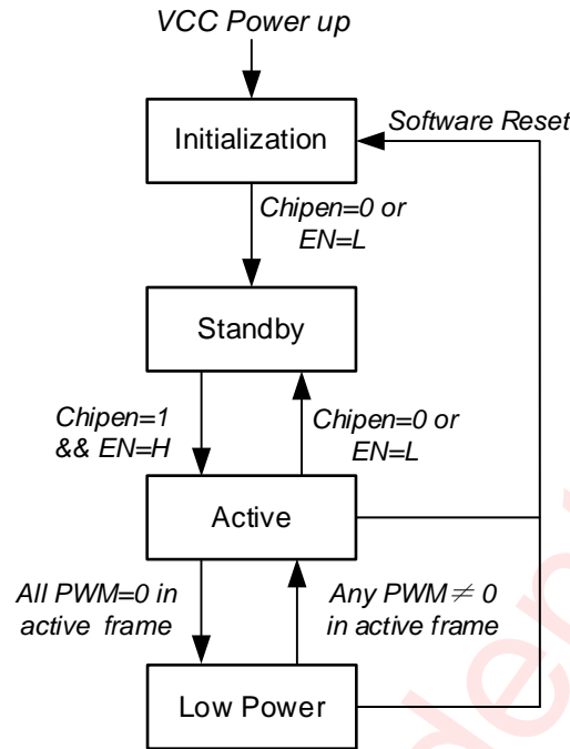
Figure 10 AW20198SG Operating Mode Transition
