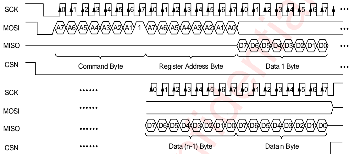
Figure 14 SPI Read from AW20198SG (Automatic Address Increment)
