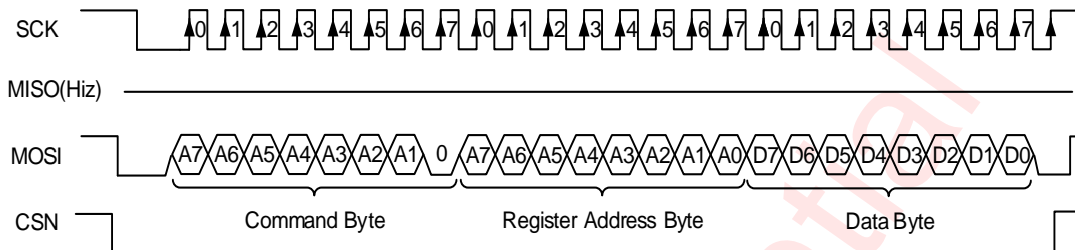
Figure 11 SPI Writing to AW20198SG (Typical)
