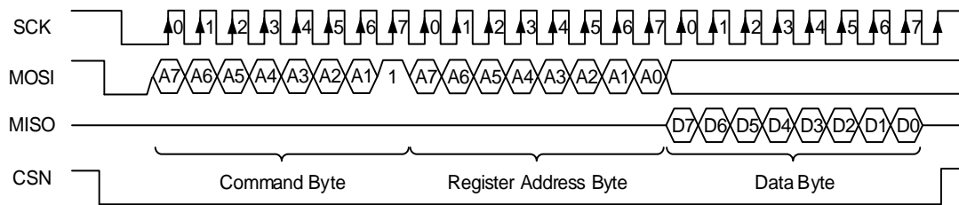
Figure 13 SPI Read from AW20198SG (Typical)
