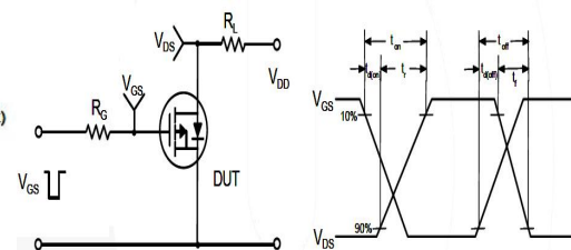
Fig15. Switching Time Test Circuit and waveforms
