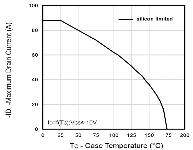
Fig12. Maximum Drain Current Vs. Case Temperature
