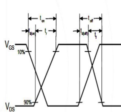
Fig15. Switching Time Test Circuit and waveforms
