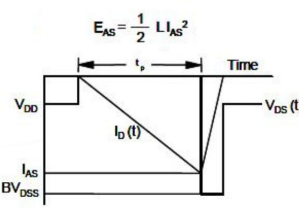
Fig14. Unclamped Inductive Test Circuit and waveforms
