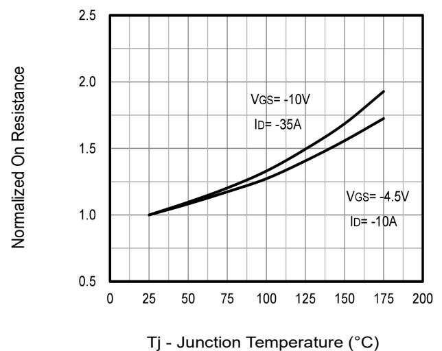
Fig4. Typical Normalized On-Resistance Vs. T_j
