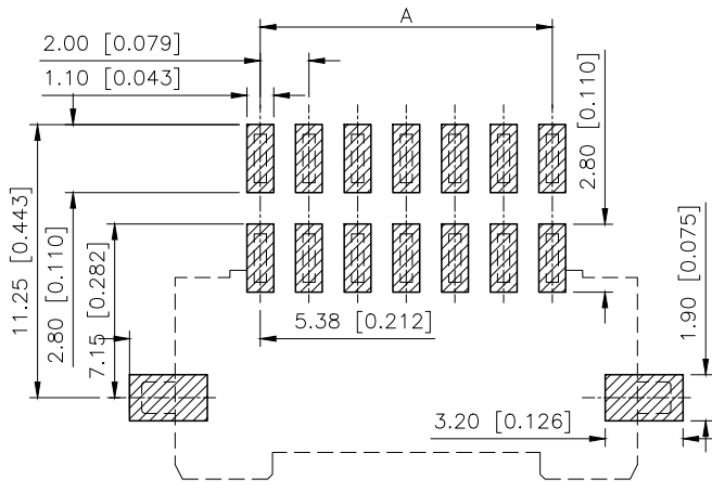
PCB LAYOUT
