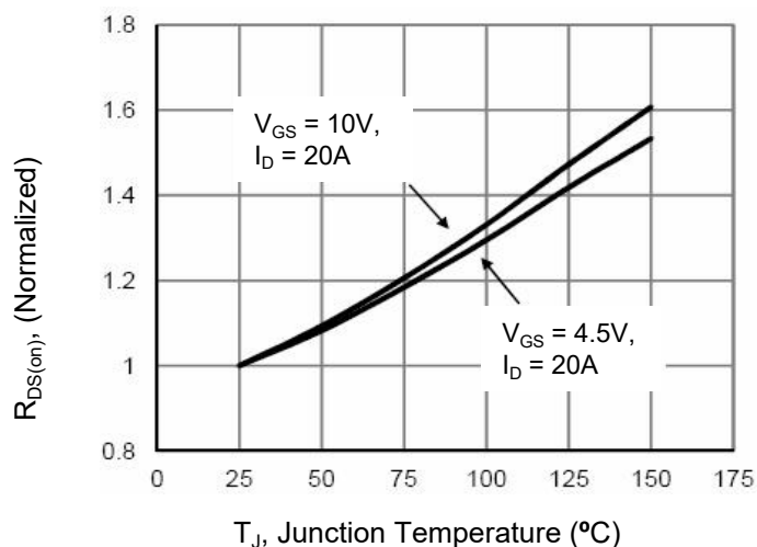
Figure 7. Drain-Source On-Resistance
