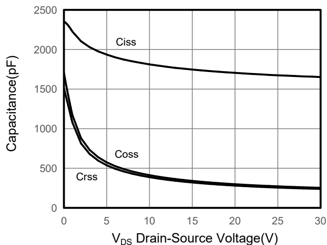
Figure 5. Capacitance
