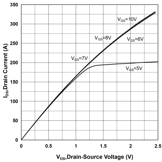
On-Region Characteristic@125°C
