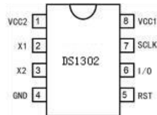
SOP-8(SOIC-8)
