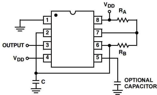
FIGURE 2B. ALTERNATE ASTABLE CONFIGURATION
