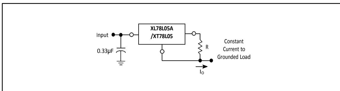
Figure 6-1. Current Regulator
