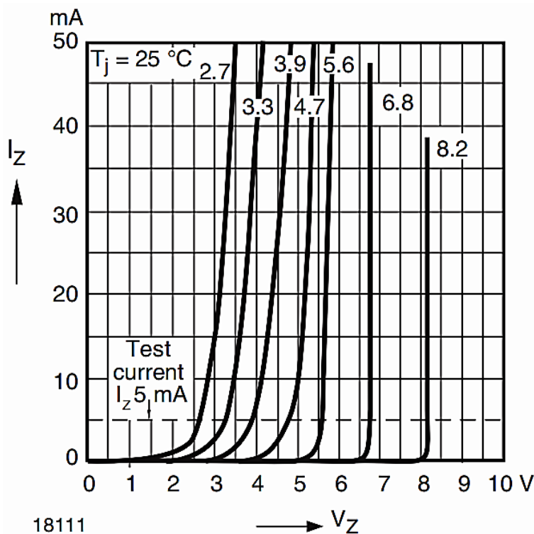
Figure 14. Breakdown Characteristics
