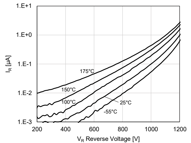
Figure 4. Reverse Characteristics
