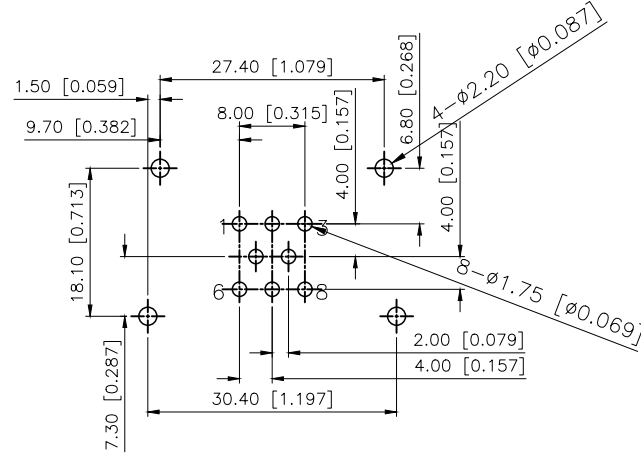
PCB LAYOUT
