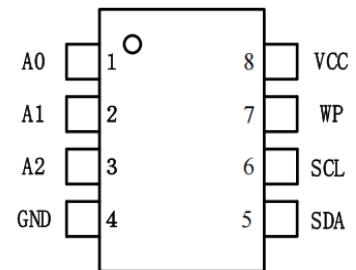
8-lead TSSOP
