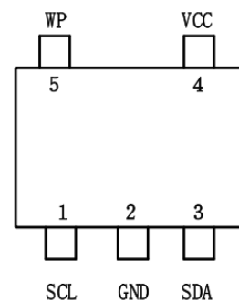
5-lead SOT23-5
