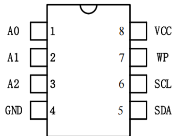
8-lead PDIP
