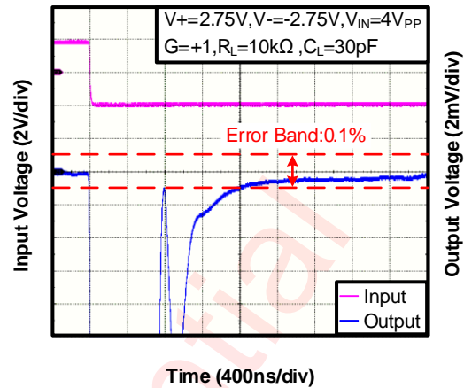
Figure 30 Large Signal Settling Time (Negative)
