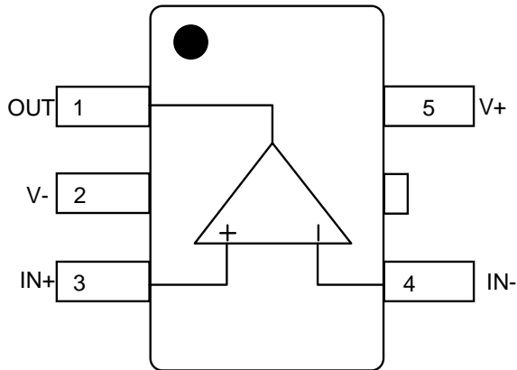
AWS79061STR (Top View)
