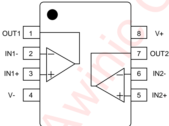
AWS79062MPR (Top View)
