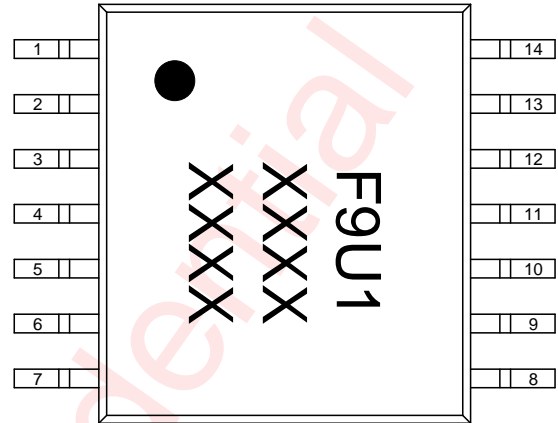
AWS79064SPRT Marking (Top View)
