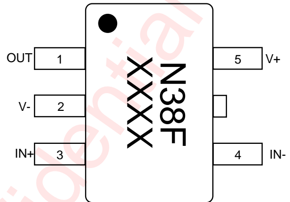
AWS79061STR Marking (Top View)
