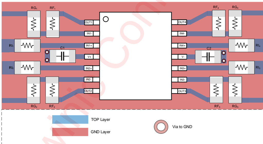
Figure 38 AWS7906X Layout Example
