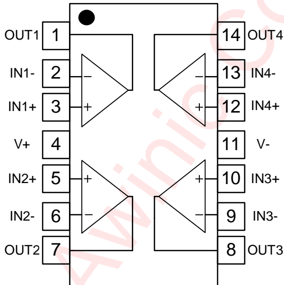
AWS79064SPR (Top View)
