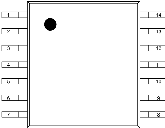
AWS79064SPRT (Top View)
