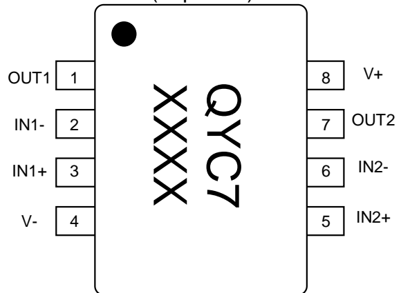
AWS79062MPR Marking (Top View)
