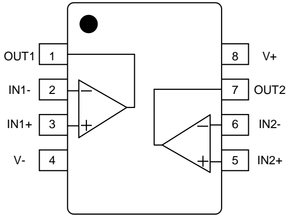
AWS79062SPR (Top View)
