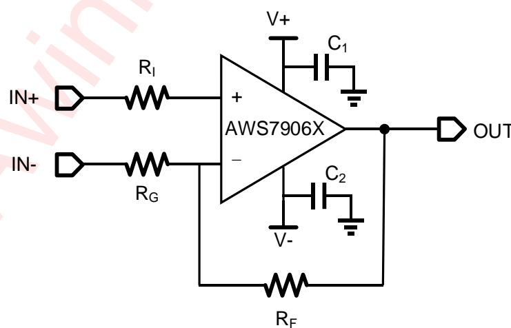
Figure 37 AWS7906X Schematic Example
