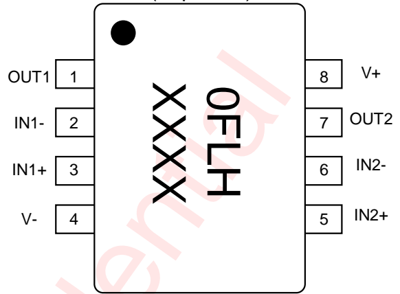
AWS79062SPR Marking (Top View)
