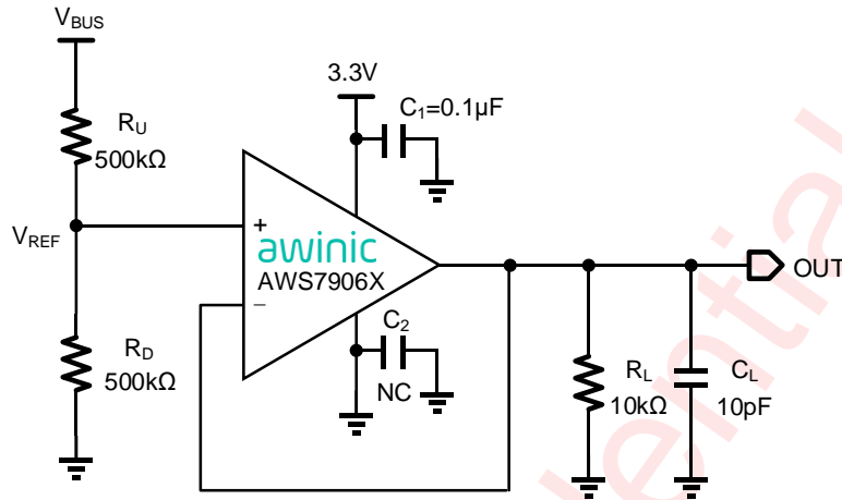
Figure 4 AWS7906X Application Circuit
