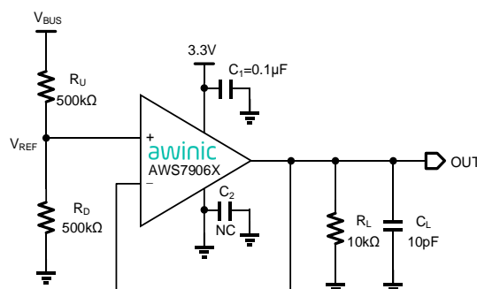
Figure 1 Typical Application of AWS7906X
