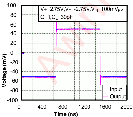
Figure 27 Small Signal Step Response
