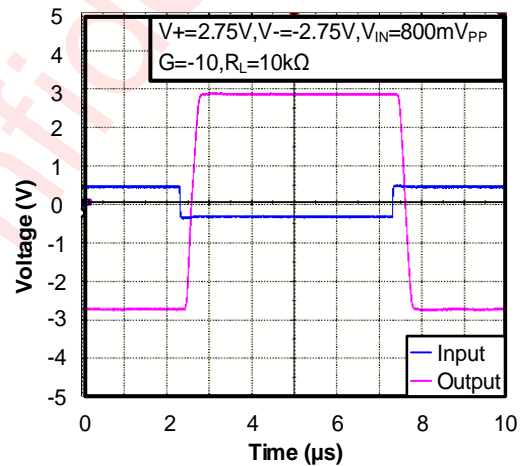
Figure 26 Overload Recovery
