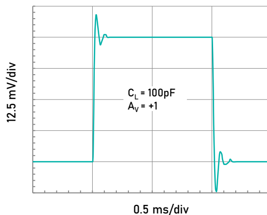
Small Signal Step Response (50mV Step).
