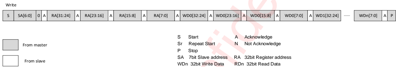
Figure 10 I 2 C Write Byte Cycle
