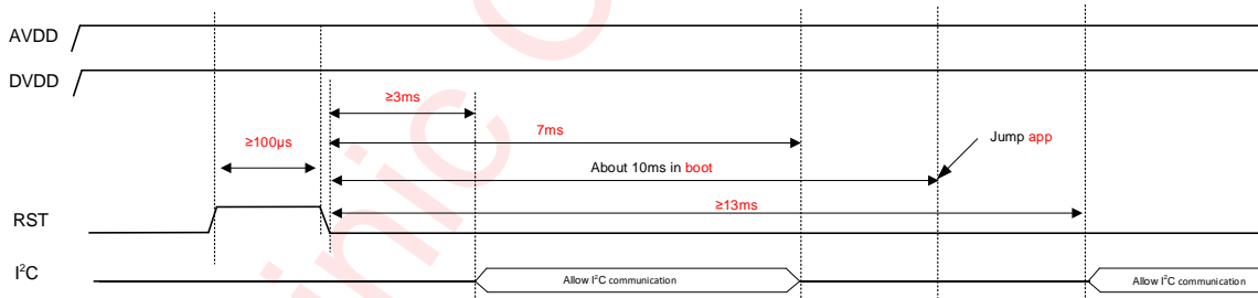
Figure 13 RST Sequence
