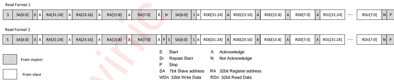
Figure 11 I 2 C Read Byte Cycle
