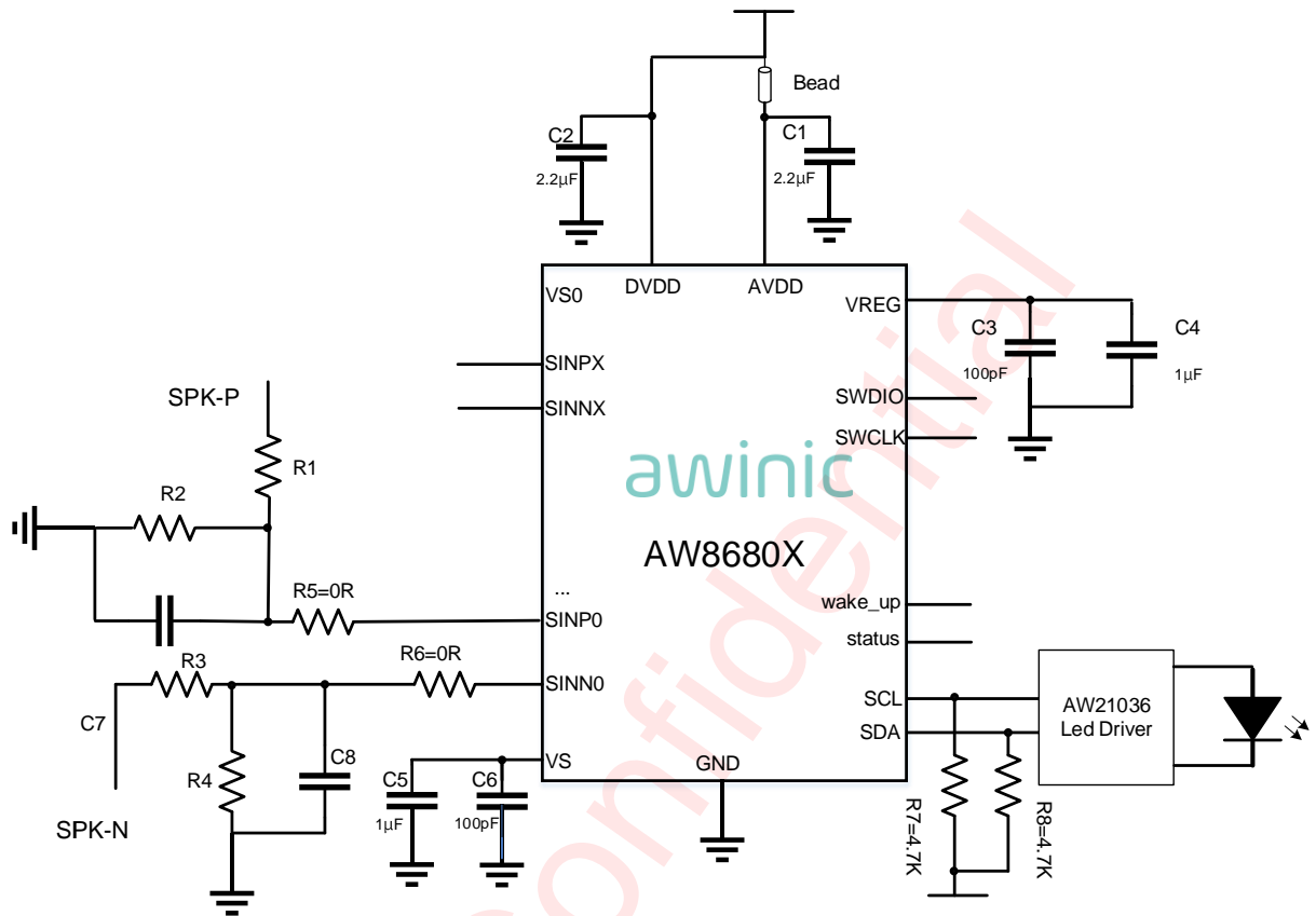
Figure 3 AW8680X Typical Application Circuit for light synchronized with sound
