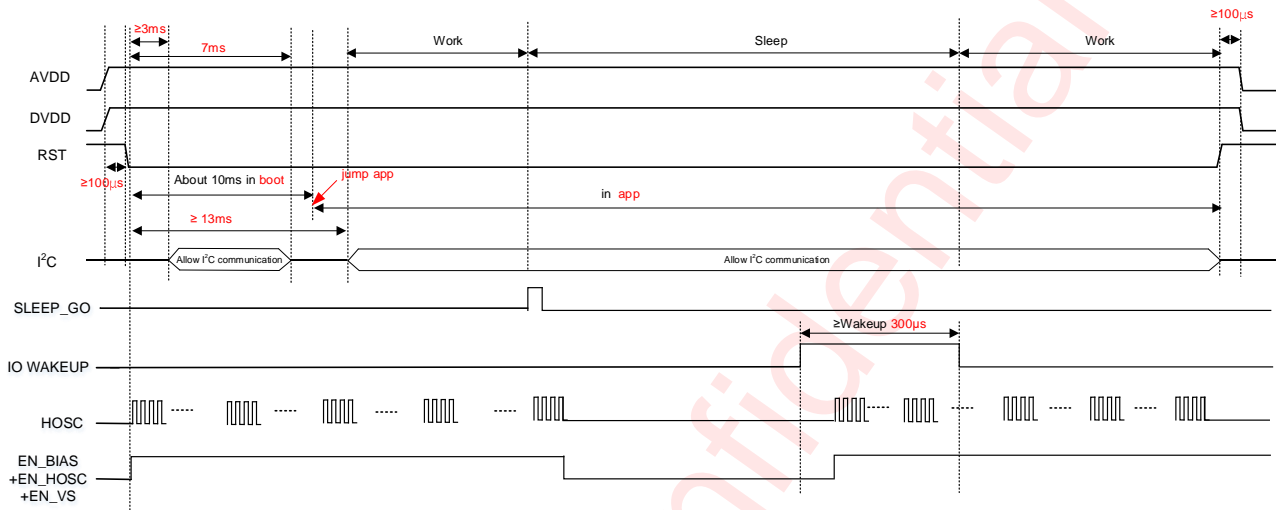
Figure 12 Power On and Power Down Sequence
