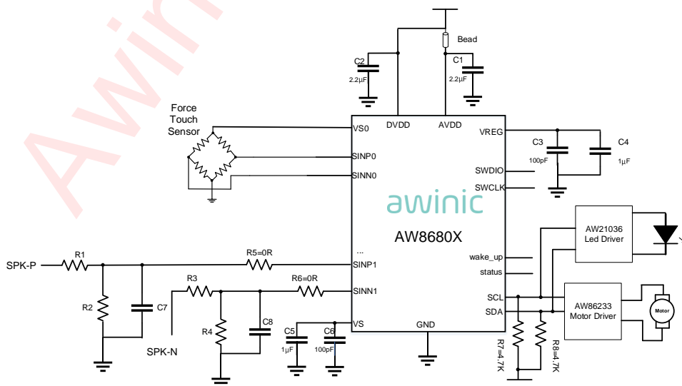
Figure 1 AW8680X Typical Application Circuit
