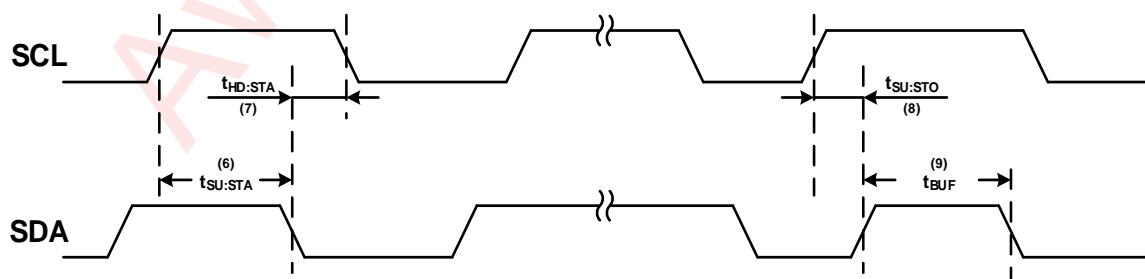
Figure 8 SCL and SDA timing relationships in the data transmission process
