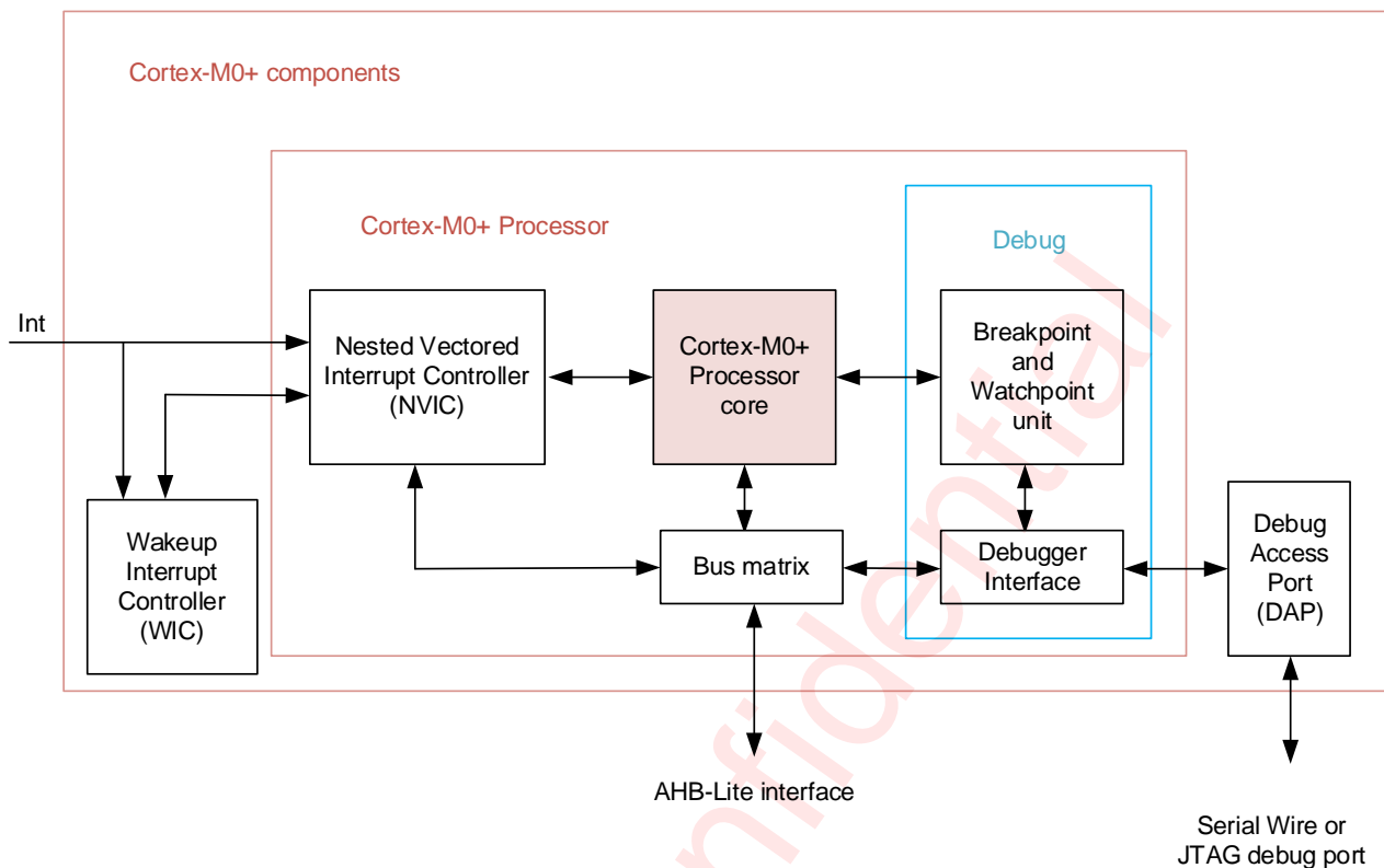
Figure 14 Cortex-M0+ core
