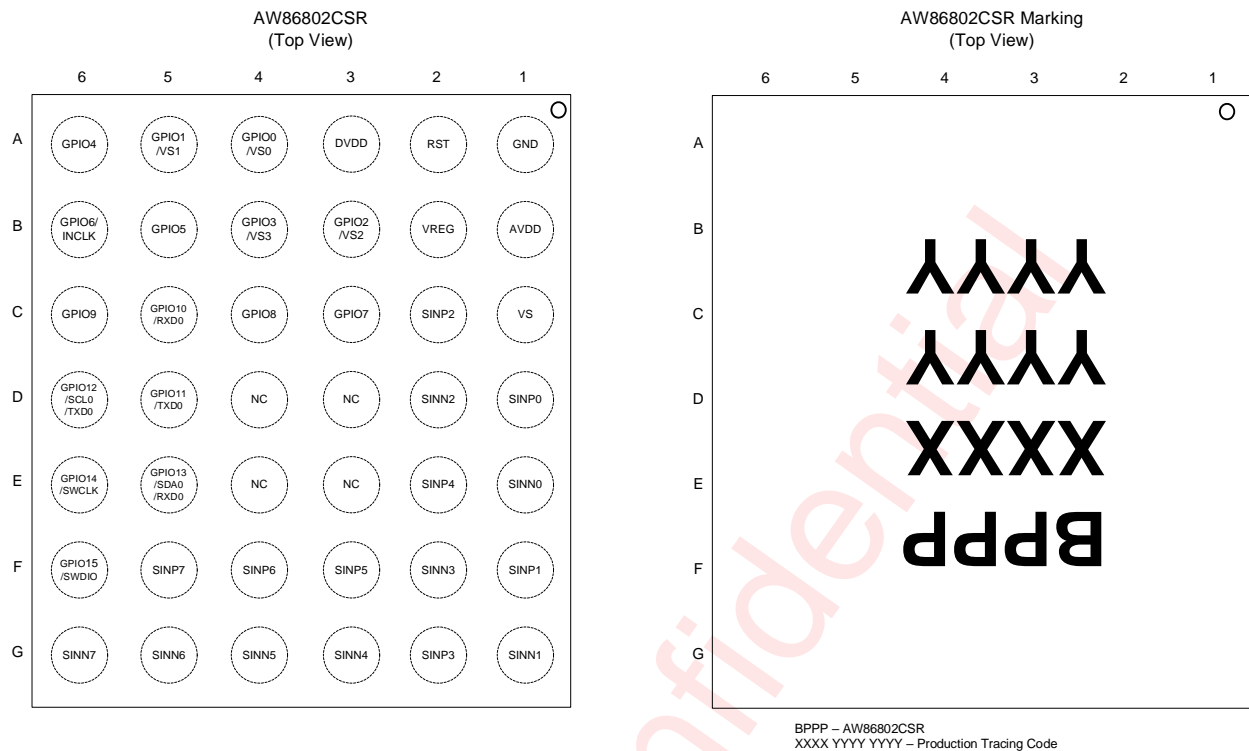
Figure 5 AW86802 Pin Configuration and Top Mark
