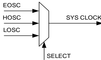
Figure 15 Clock
