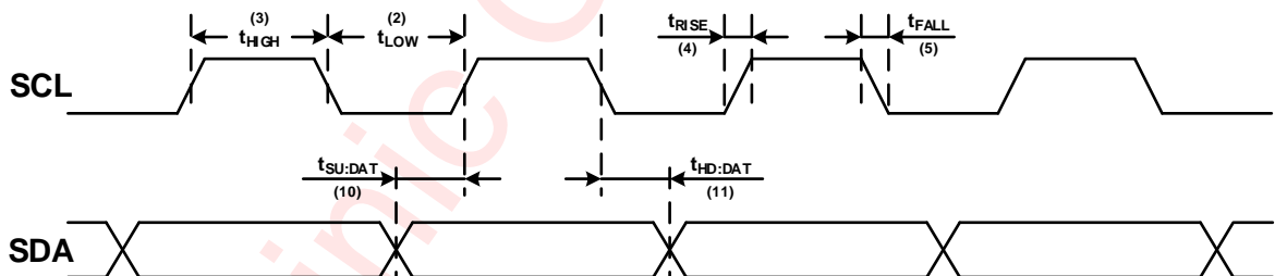
Figure 8 SCL and SDA timing relationships in the data transmission process
