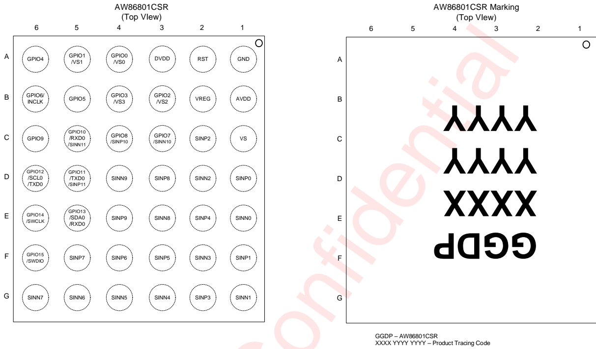
Figure 4 AW86801 Pin Configuration and Top Mark
