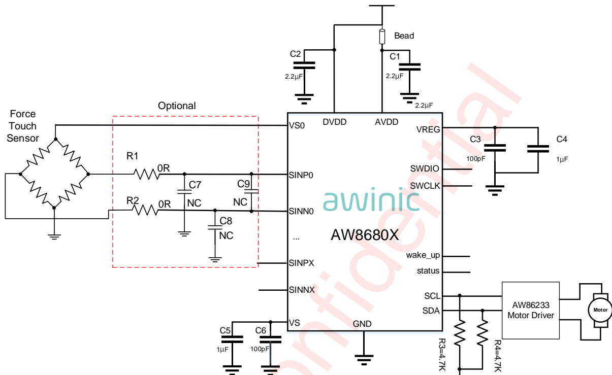
Figure 2 AW8680X Typical Application Circuit for force and E-brushtooth
