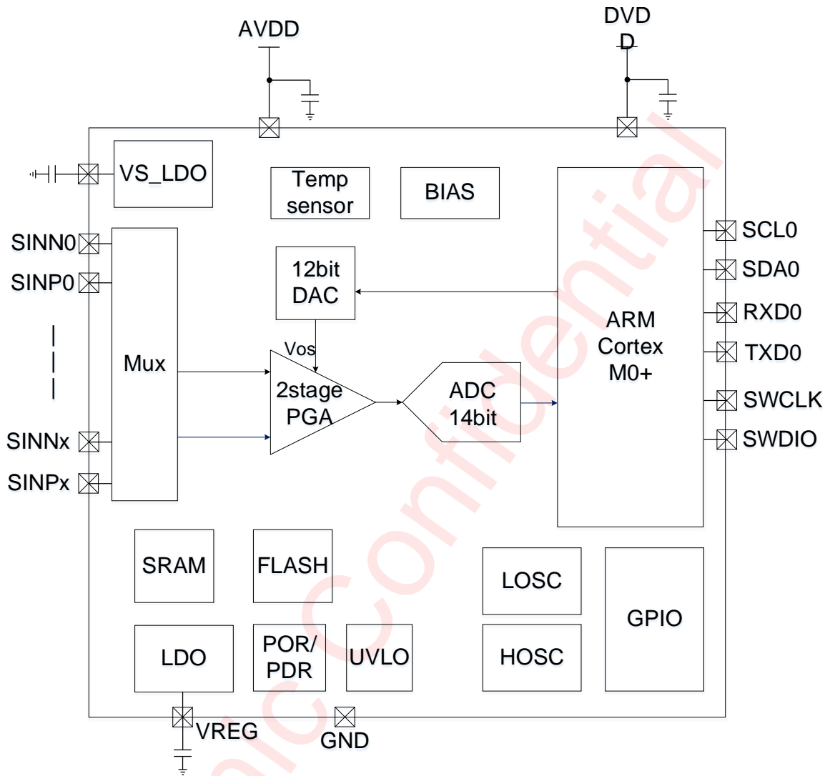
Figure 7 AW8680X Function Block Diagram
