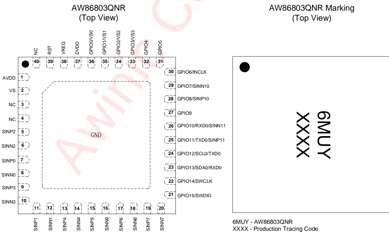
Figure 6 AW86803 Pin Configuration and Top Mark
