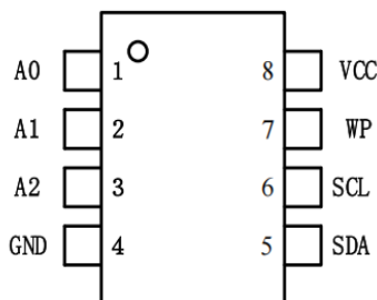
8-lead SOP
