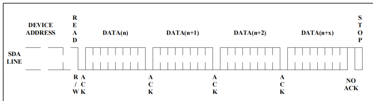
Figure 11. Sequential Read
