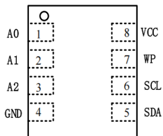
8-pad DFN
