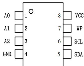
8-lead TSSOP
