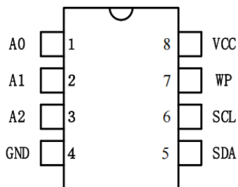
8-lead PDIP
