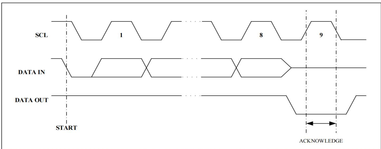
Figure 4. Output Acknowledge
