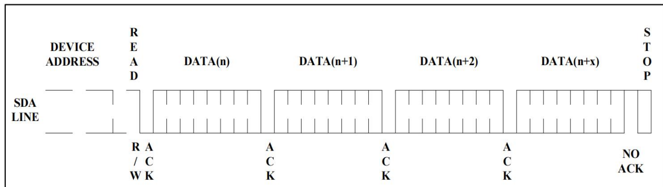
Figure 10. Sequential Read
