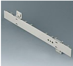
A0106280 ⓘ Side panel 0.5 HE, for handle mounting ABS (UL 94 HB) pepple gray RAL 7032 9.84"x0.88"
