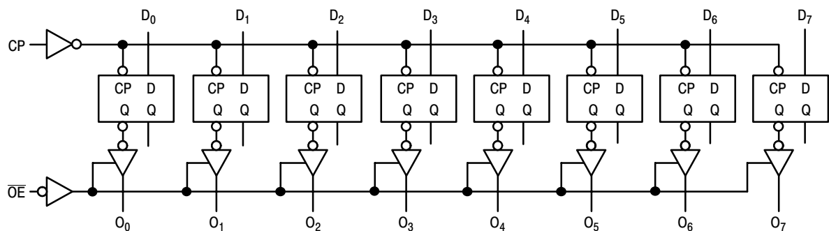
Figure 3. Logic Diagram
