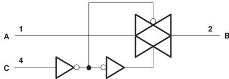
Figure 3.1: SN74LVC1G66 Logic Diagram
