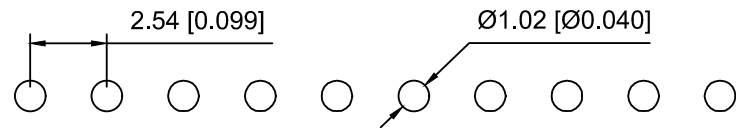
PCB LAYOUT
